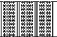
TRULINE® HP & TS 12" Soffit - Full Vent HP: SV TS: SV_BLDR Aluminum 0.019" & .016" NFA 19.6
