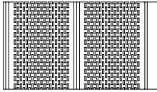
TRULINE® HP Double 6" Soffit - Full Vent D6VS Aluminum 0.019" NFA 12.0
