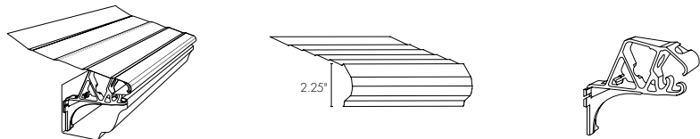
TRUGUARD® GUTTER PROTECTION KIT 5": GPP 6": GPP6 Aluminum 0.024"
