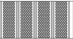
TRULINE® HP 16" Soffit - Full Vent HP: 16V Aluminum 0.019" NFA 19.1
