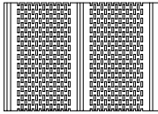
TRULINE® HP Double 5" Soffit - Full Vent D5VS Aluminum 0.019" NFA 12.0
