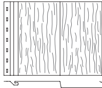
5" x 5" Board & Batten 5X5BBS & 5X5BBSHD2 Steel 0.016"
