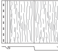
5" x 5" Board & Batten 5X5BBS & 5X5BBSHD2 Steel 0.016"
