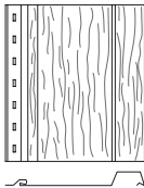
6" Board & Batten 6BBS & 6BBSHD2 Steel 0.016"
