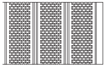
TRULINE® HP & TS 12" Soffit - Full Vent HP: SV TS: SV_BLDR Aluminum 0.019" & 0.016" NFA 19.6
