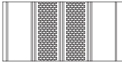
TRULINE® HP & TS 16" Soffit - Center Vent HP: 16SCV TS: 16SS_BLDR Aluminum 0.019" & 0.016" NFA 9.9
