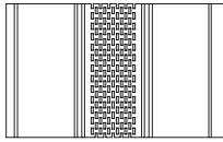
TRULINE® HP & TS 12" Soffit - Center Vent HP: CV TS: SCV_BLDR Aluminum 0.019" & 0.016" NFA 5.9
