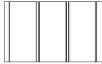
TRULINE® HP & TS 12" Soffit - Solid HP: S TS: S_BLDR Aluminum 0.019" & 0.016"
